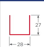
Ref. Poste T S60 1.2mm - TC PL-S60-TC-PST-12
