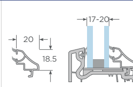
Junquillo 17-20mm S60
