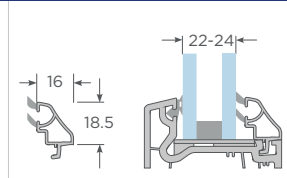
Junquillo 22-24mm S60
