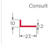
Ref. Contra Flecha 2mm - TC PL-CMP-TC-CTF-2
