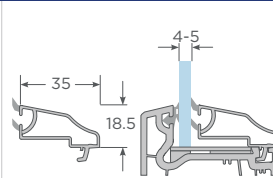
Junquillo 4-5mm S60
