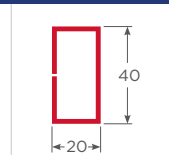
Ref. Inercia T 2mm - TC PL-CMP-TC-INT-2
