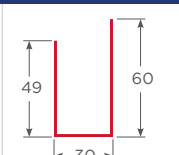
Ref. Hoja Puerta S60 1.5mm - TC PL-S60-TC-HPF-15
